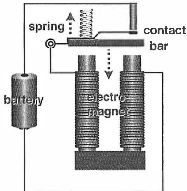
Electric buzzer
